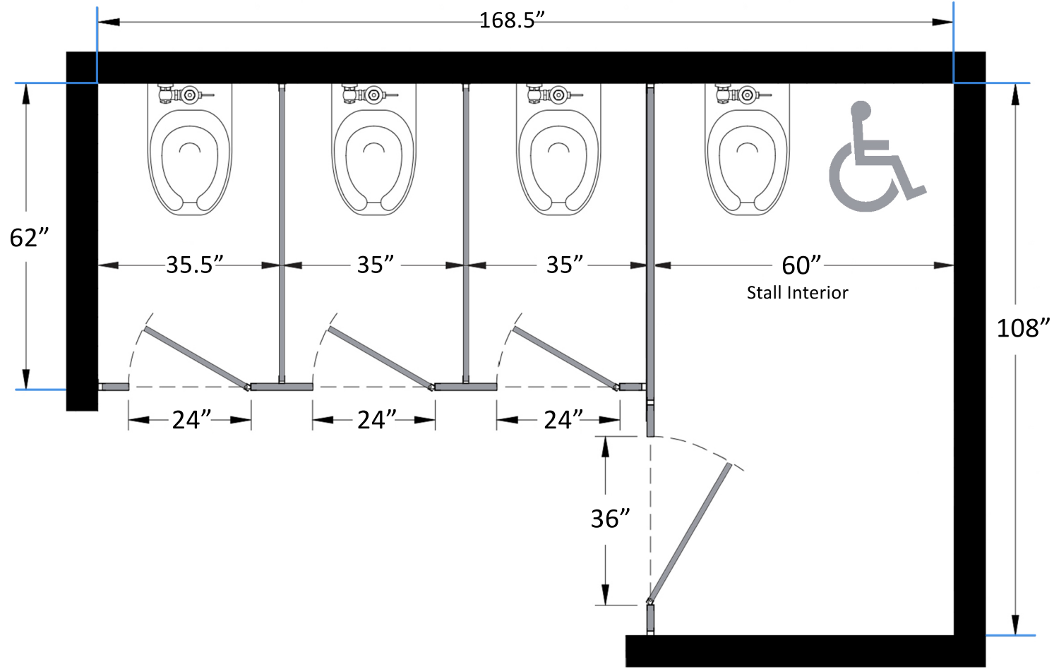
Bathroom Partitions - 4 Stall Alcove Right Hand SKU: AL4R Standard Dimensions
